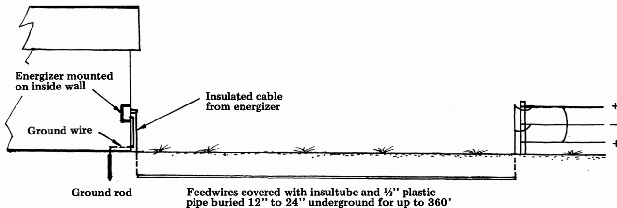
Underground transmission from energizer to fence.
