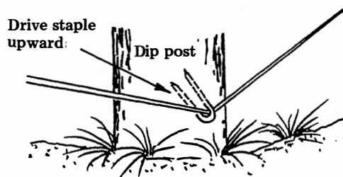
Stapling guide wire to dip post.
