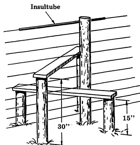
People-access stile.
