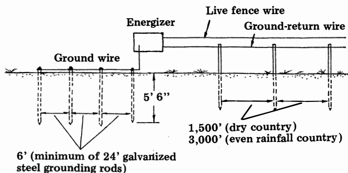
Grounding fence.
