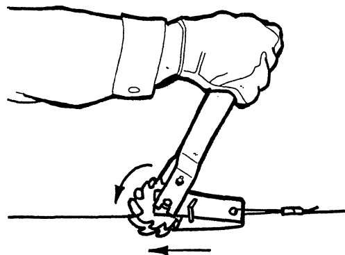
Tighten wire with in-line strainer.
