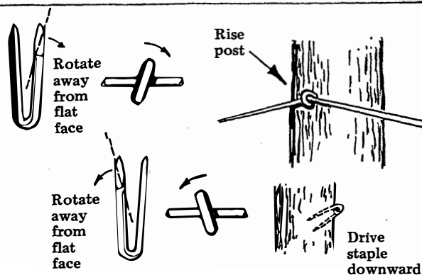
Proper methods of stapling.
