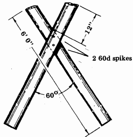
Framing horse for jack leg of buck mortice joints
