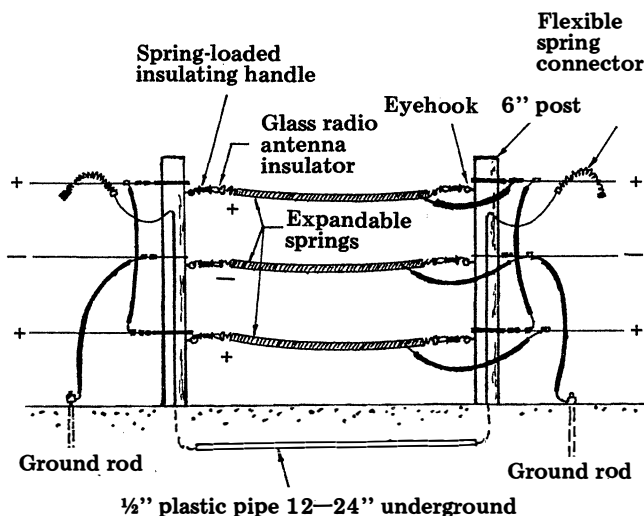
Expandable spring gate.
