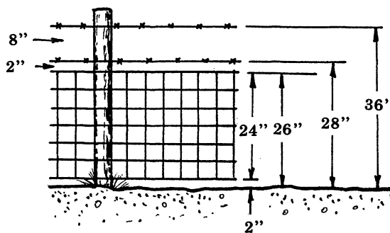
Woven wire with 2 strands barbed wire
