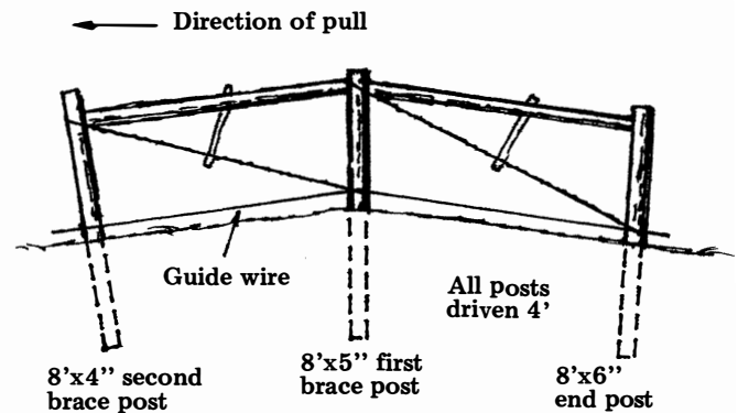
Brace construction for high tensile fences of seven or more wires.
