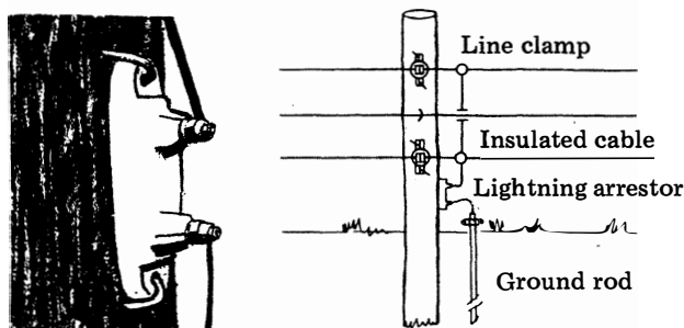
Lightning arrestor.
