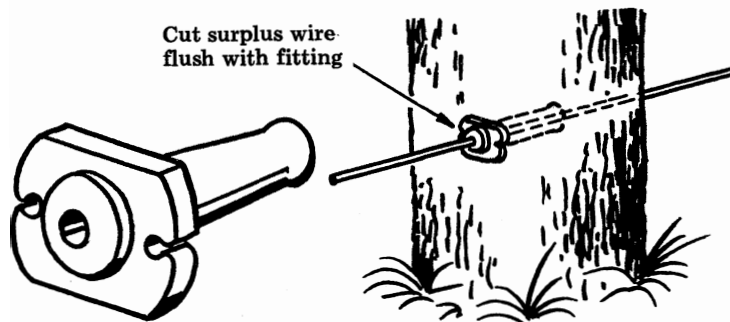
Using Reliable Wirevise R to fasten wires to end, corner and gate posts.
