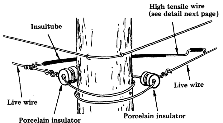
Disconnectable joint.
