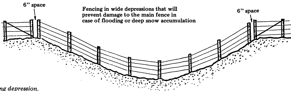
Fence crossing depression.
