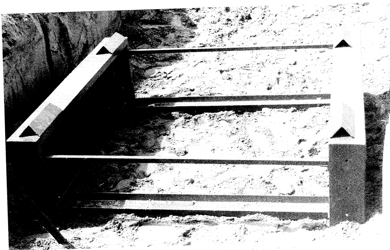
Typical steel foundation cattleguard under construction.
