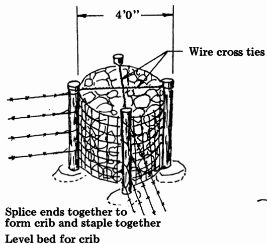
Rock crib corner post
