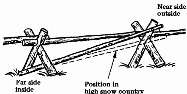
Method of attaching diagonal brace to the bucks.
