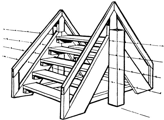
Fence stile.
