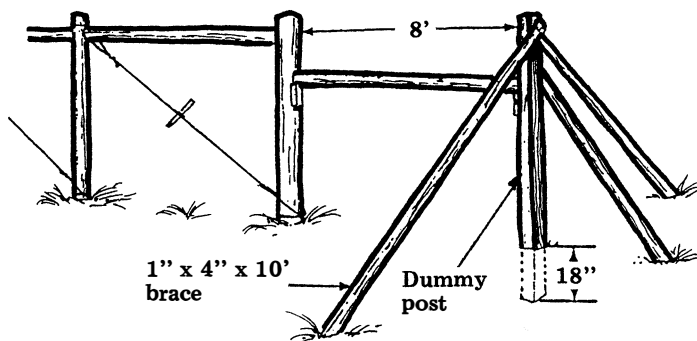
Dummy post details.
