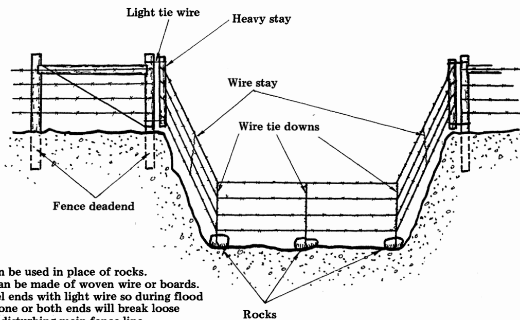
Brace design and placement considering changes in topography.
