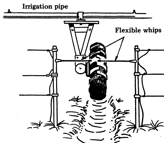
Pivot irrigation system gate.
