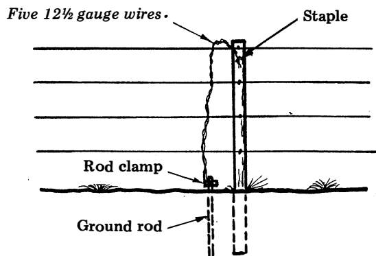
Grounding fence.
