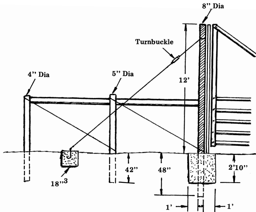
Double panel gate brace.
