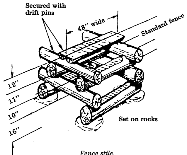
Fence stile.
