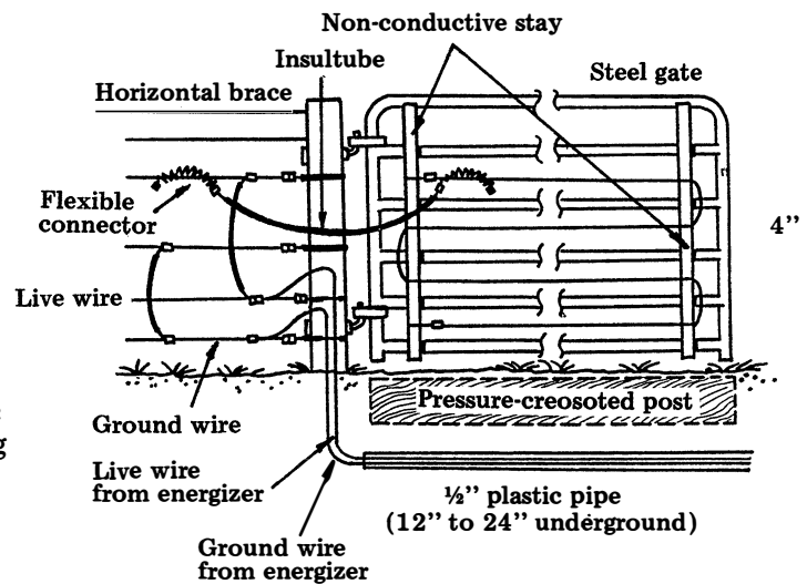
Electrified conventional gate.
