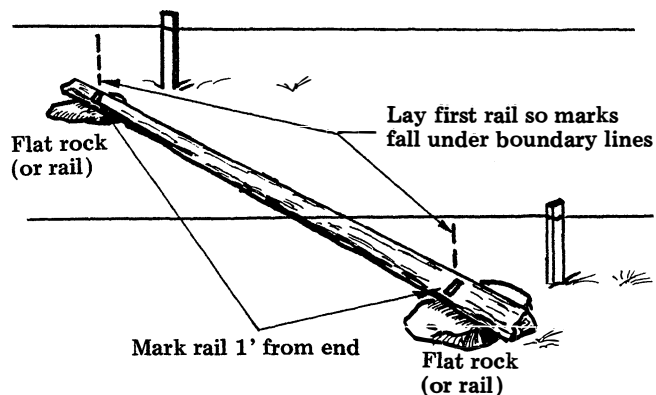
Laying the bottom rail.
