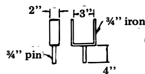
STIRRUP FOR GATE POST
