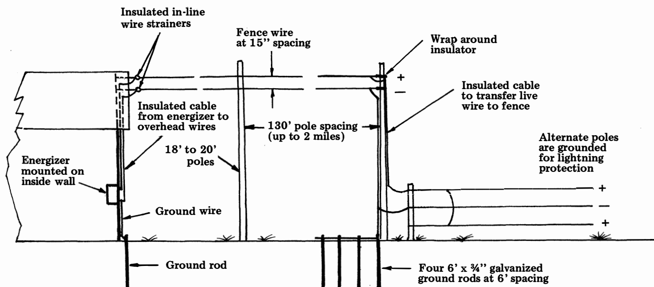
Overhead transmission from energizer to fence.
