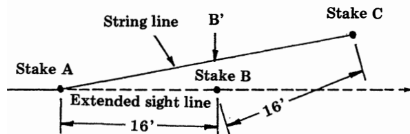
Rounding a shallow one post curve.
