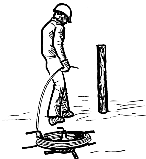
A rotating payout reel is used to string the guide wire.
