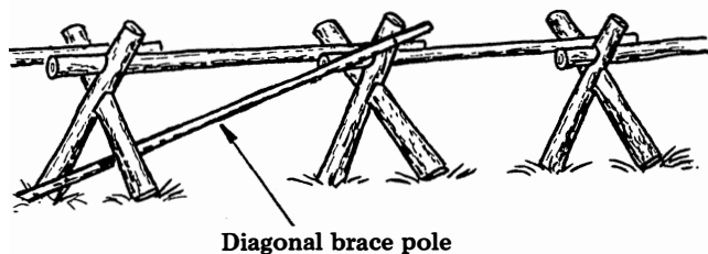
Adding diagonal brace poles for rigidity.
