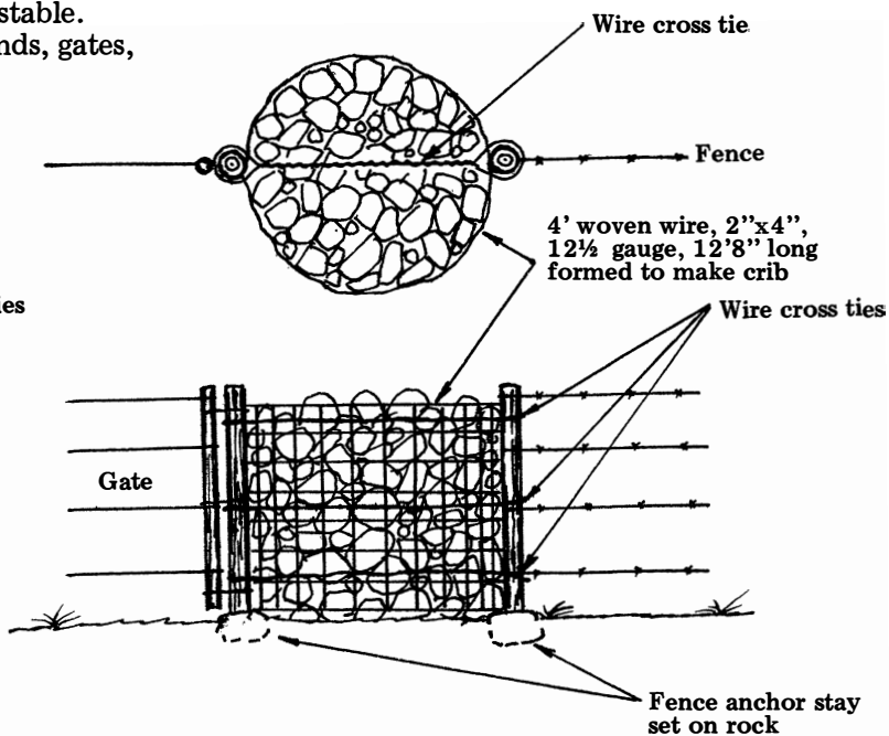
Rock crib gate post
