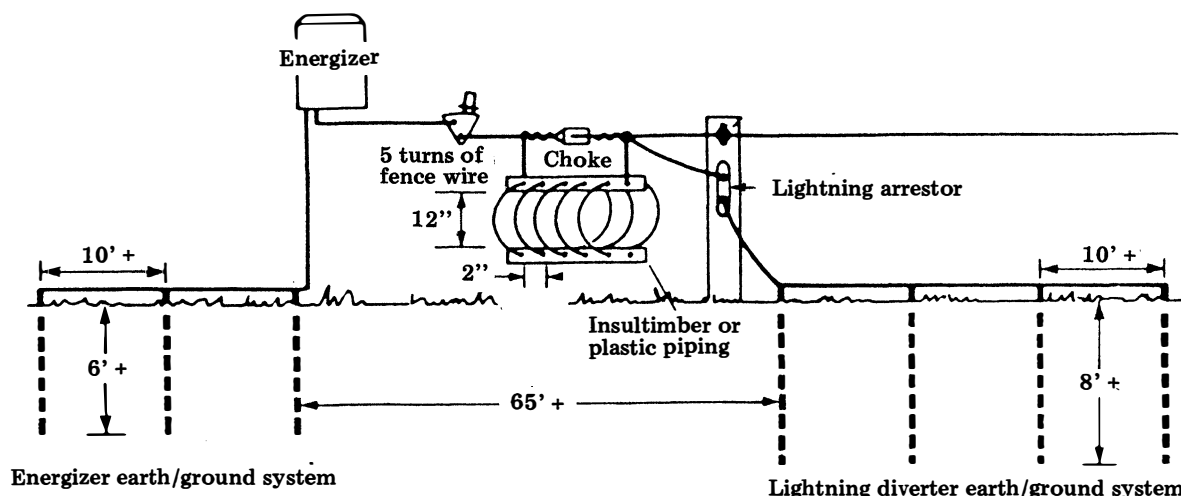
Choke assembly.
