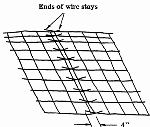
Splicing a net fence.
