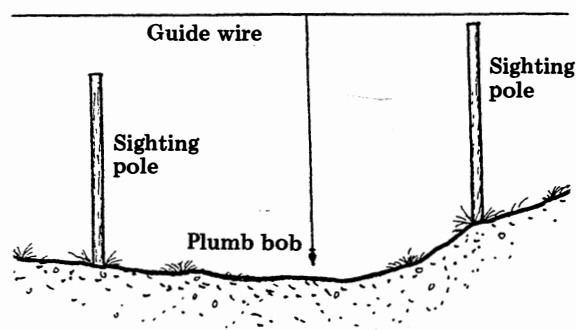
Marking dip post location.
