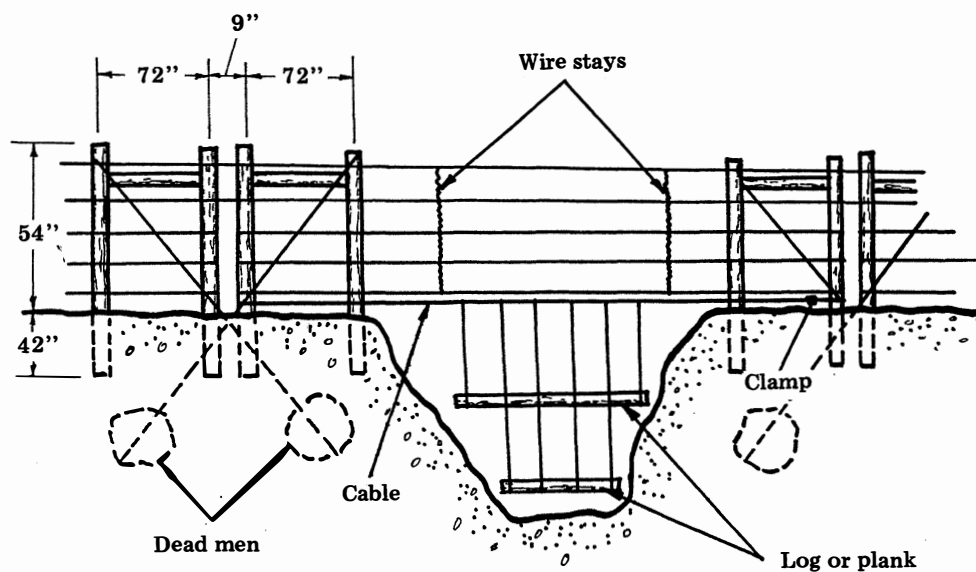
Water gap for narrow drainages.
