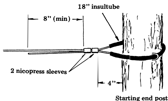
Bottom wire tie off.
