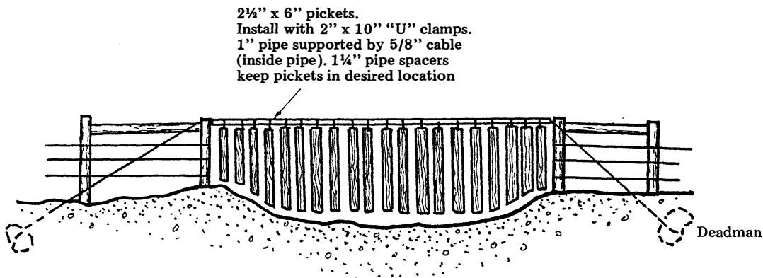
Picket fence across streams.
