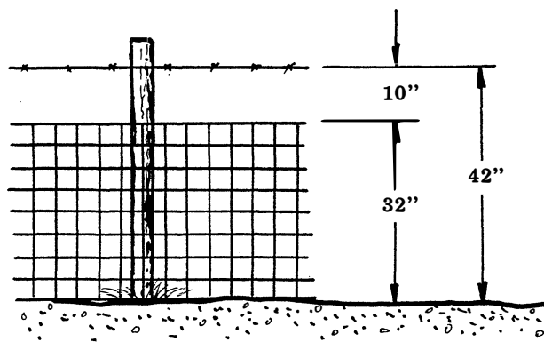
Woven wire with 1 strand barbed wire
