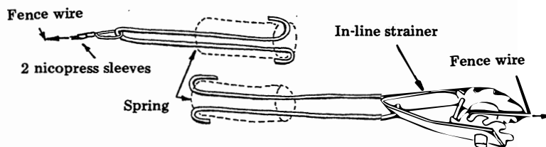
Installing in-line adjustable wire strainer.
