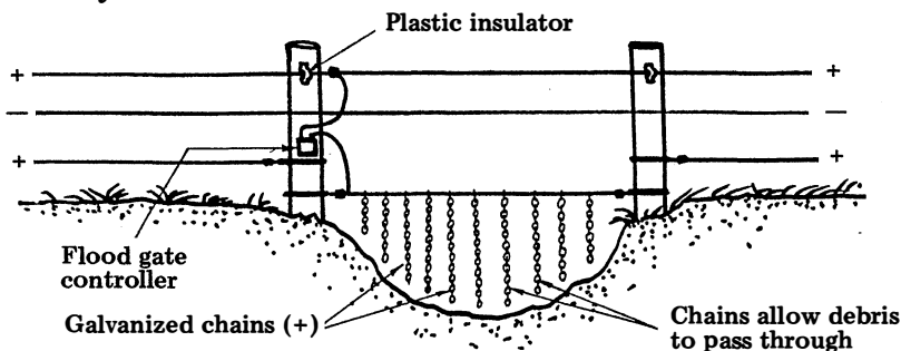
Electric flood gate.
