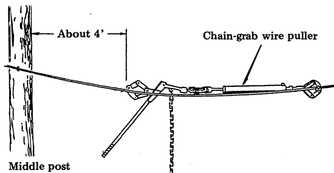
Pulling slack from wire.
