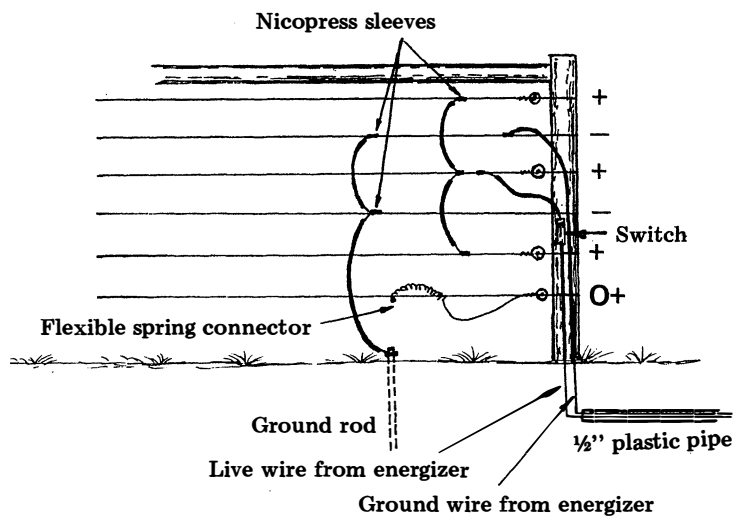
Typical diagram of electrical connections.
