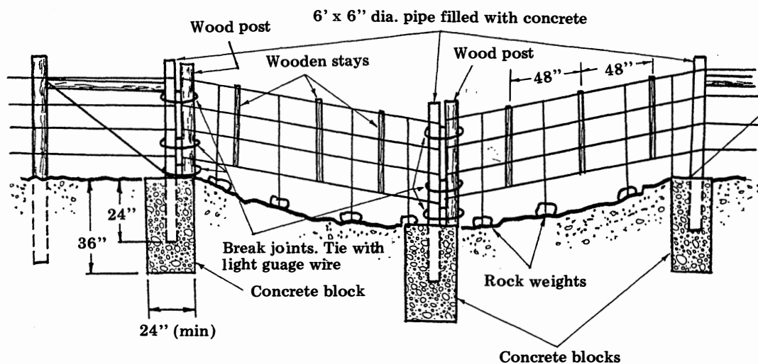
Break-away fence for wide, shallow water gaps.
