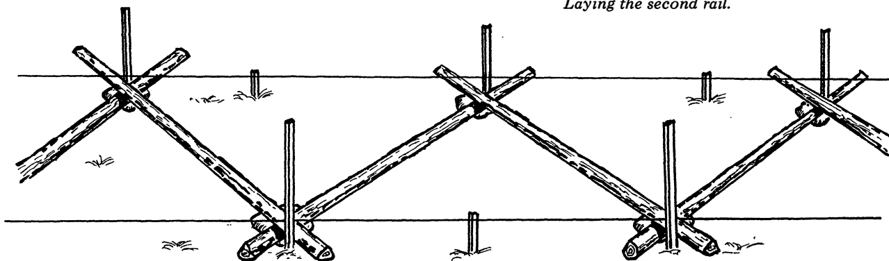
Continue laying bottom and second rails for the entire fence line.
