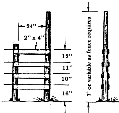
Standard fence post
