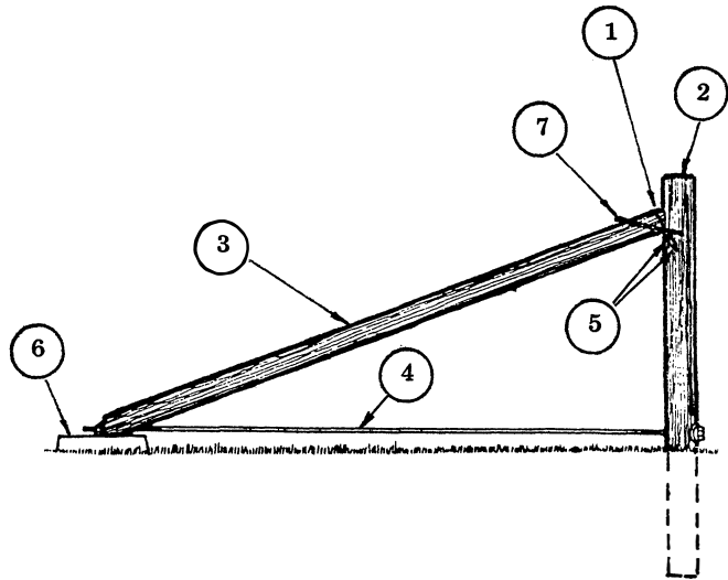
Kiwi diagonal with a float foot.
