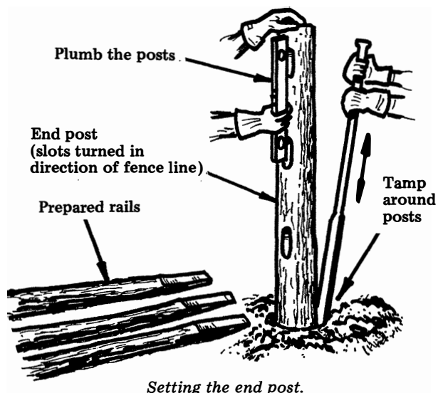
Setting the end post.
