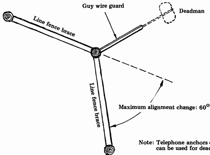
Angle guy with deadman.
