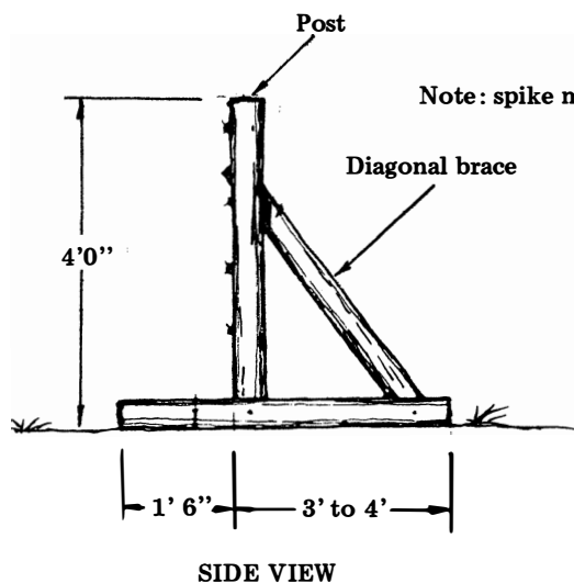
Figure-4 post.
