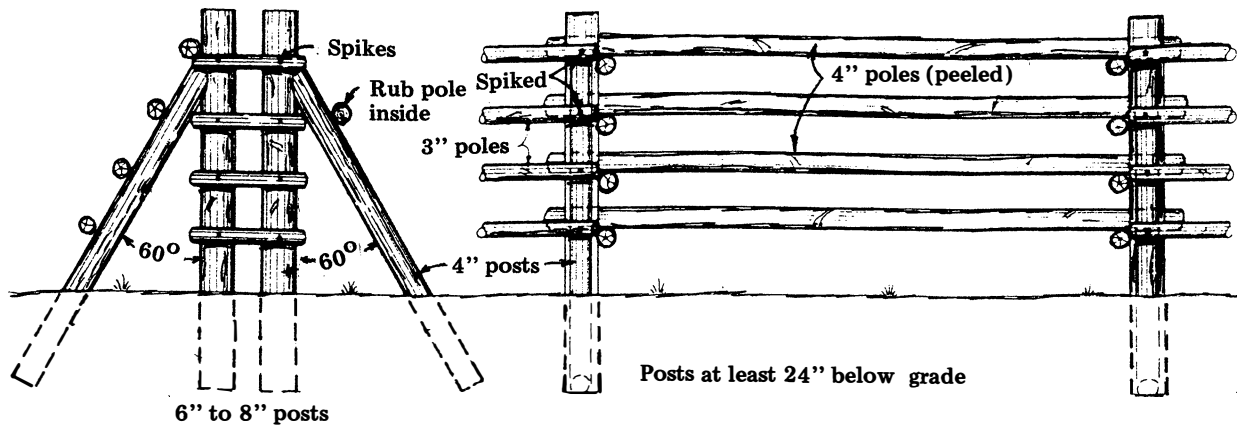
SECTION THROUGH GATE
