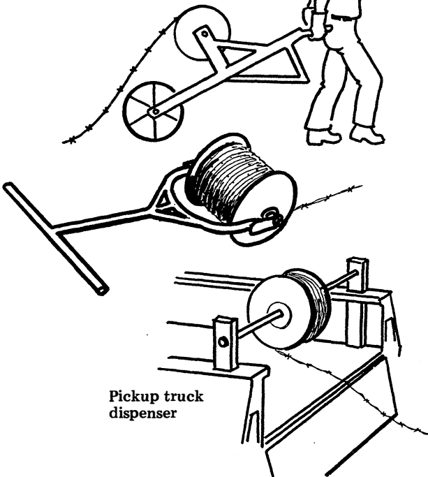
Home-made unrolling devices
