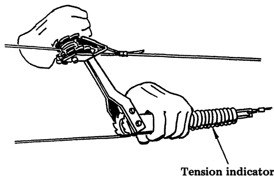
Installing tension indicator.
