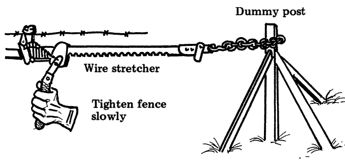
Stretching barbed wire.
