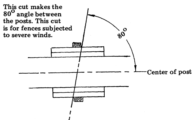
Cutting 60° and 80° angles on posts.
