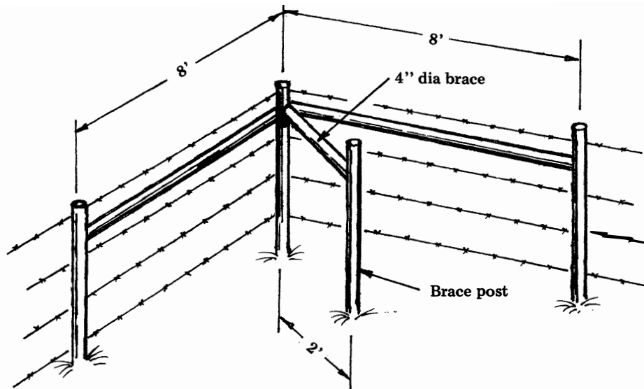
Interior horizontal deadman.
