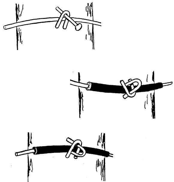
Temporary wire stapling.
