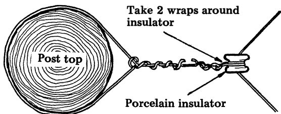
Tying on inside corner using New Zealand knot.
