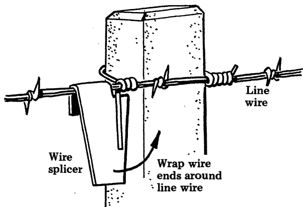
Using wire splicer to attach wire to concrete post.
