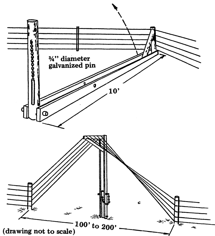
Multiple wire lift gate.
