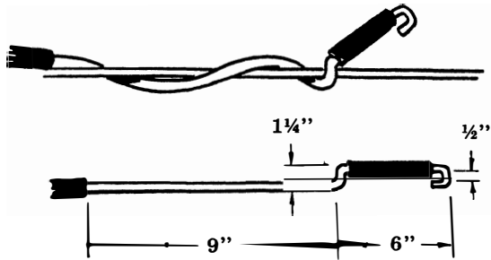
Disconnectable joint detail.
