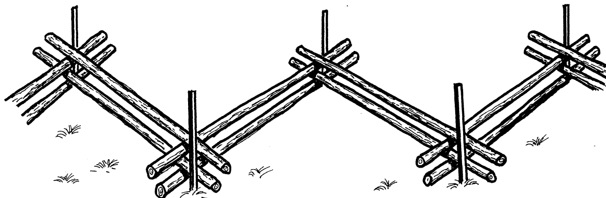
Stacking other rails (use 5-foot stakes for guides).
