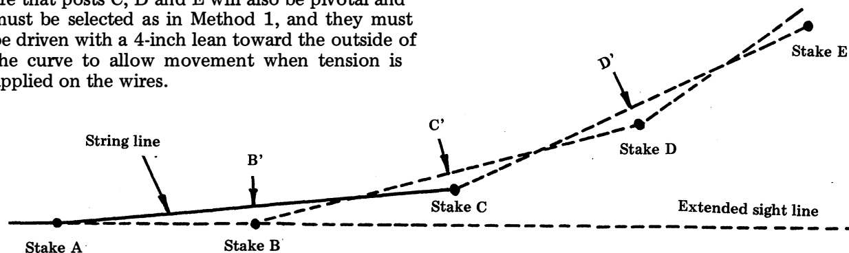
Rounding a long gradual curve.
