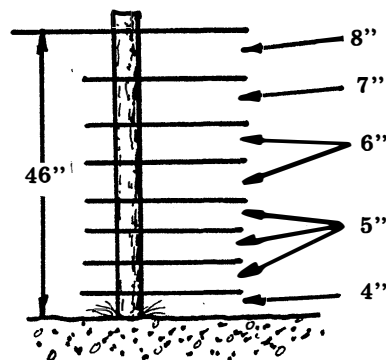
RANGE 8-STRAND BOUNDARY FENCE
