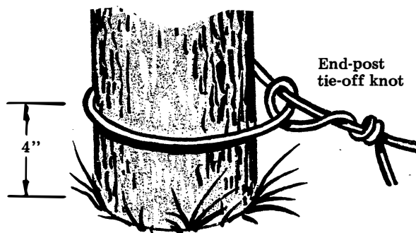
Wrapping wire at far end post.
