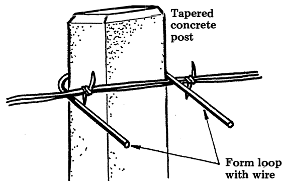
Fastening wire to tapered concrete post.
