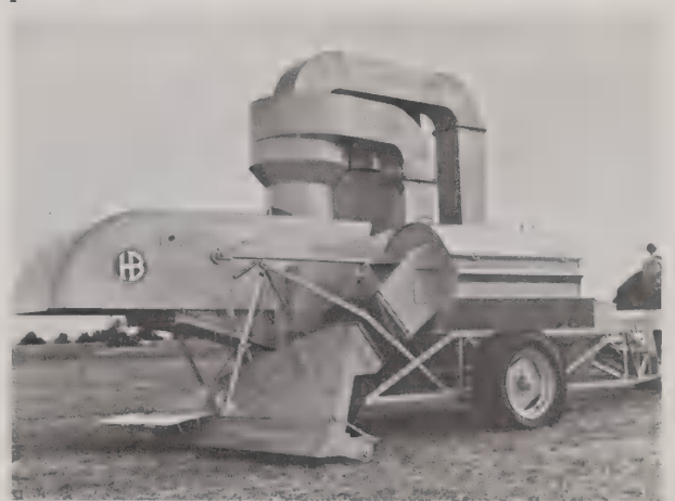
Horwood Bagshaw, Ltd.'s Universal Seeds Harvester with large threshing cylinder.
